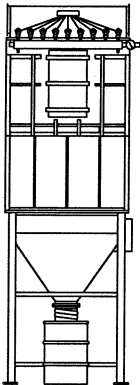
JET BAG
