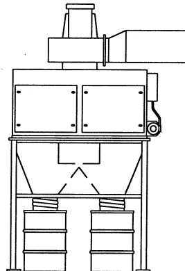
FILTER BAG
